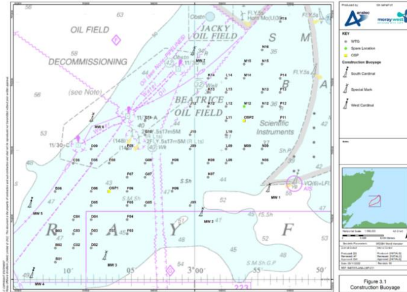
Figure 5: Layout of demarcation Buoyage
