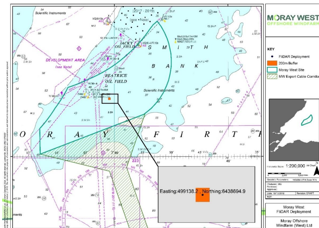
Floating LiDAR Buoy Original Site Location
